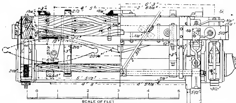
Fig. 4815. Half Cross Section and Half End Elevation. PASSENGER-CAR TRUCK, FOUR-WHEELED. NEW YORK, LAKE ERIE & WESTERN RAILROAD.
